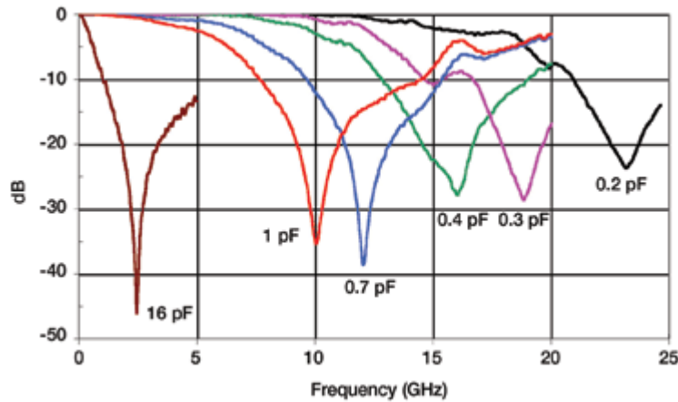
Fig. 2. S21 forward transmission loss characteristics curve. When using a thin-film capacitor, manufacturers can reap the electrical benefits of a single-layer capacitor while being rewarded with the processing ease of an MLCC-type component. A thin-film capacitor's consistent performance impact on electrodes and oxide thickness and quality impact on dielectric K is shown in Fig. 3.
