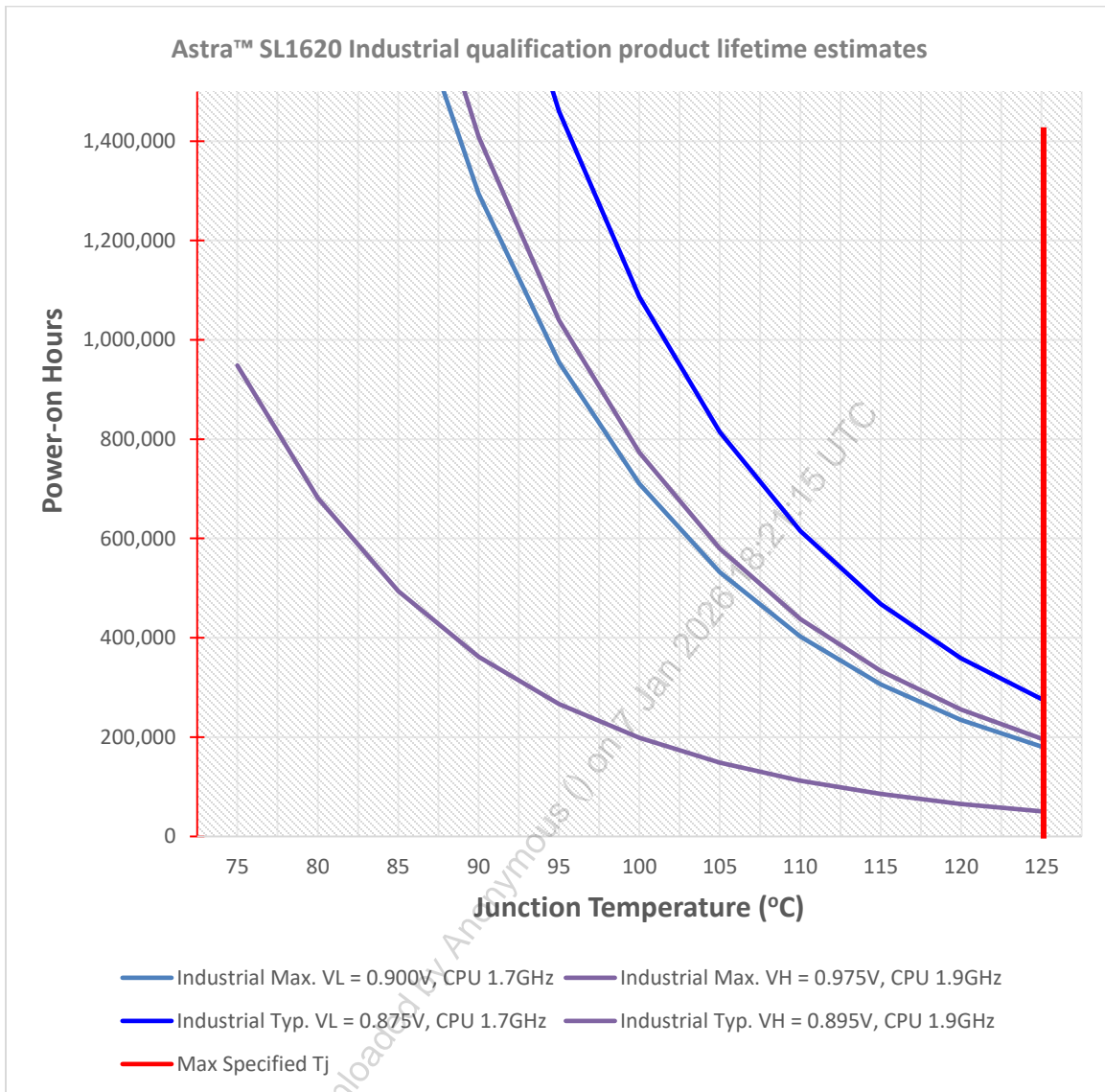
Figure 2. Astra SL1620 Industrial qualification product lifetime estimates
