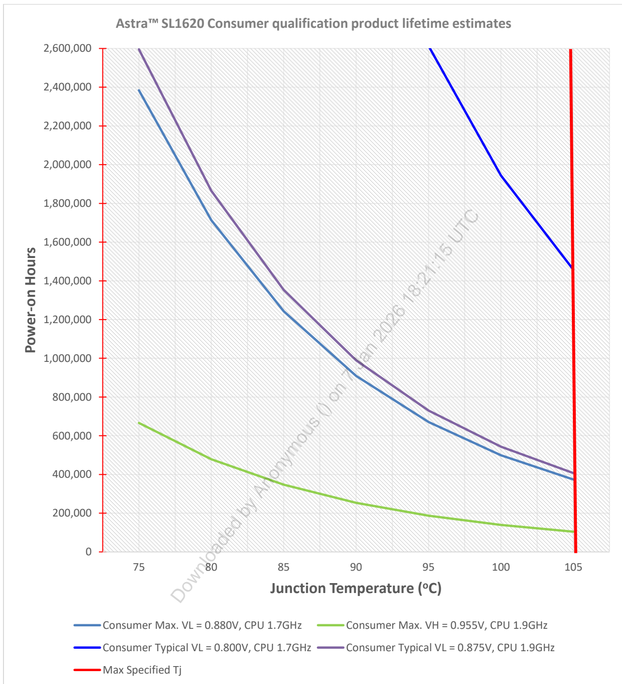
Figure 1. Astra SL1620 Consumer qualification product lifetime estimates
